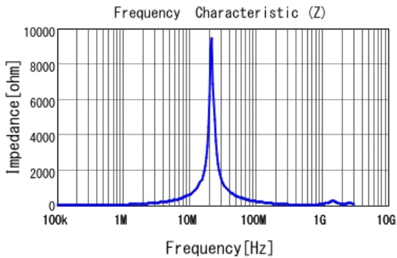
■ 1264EY-100M |Z|
