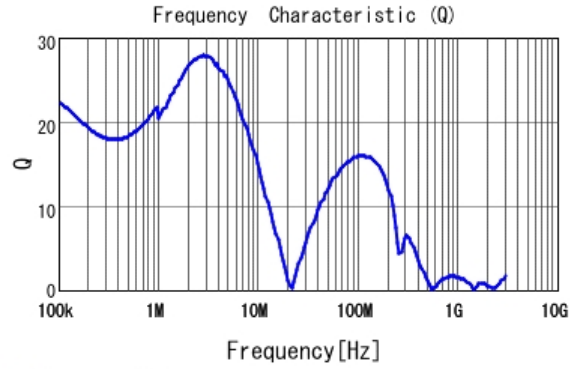
■ 1264EY-100M Q
