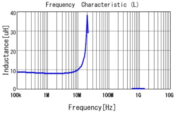
■ 1264EY-100M L
